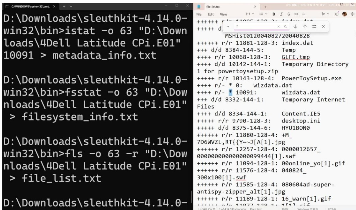
Figure 4: Searching file_list.txt to identify the deleted wizdata.dat file at inode 10091
